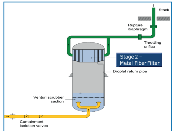
Schematic of Framatome's FCVS Standard
