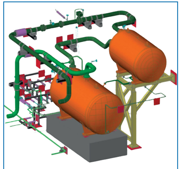
3D model of a split vessel design of Framatome's FCVS Standard
