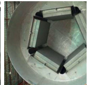
Example of Stage 2 Metal Fiber Filter
