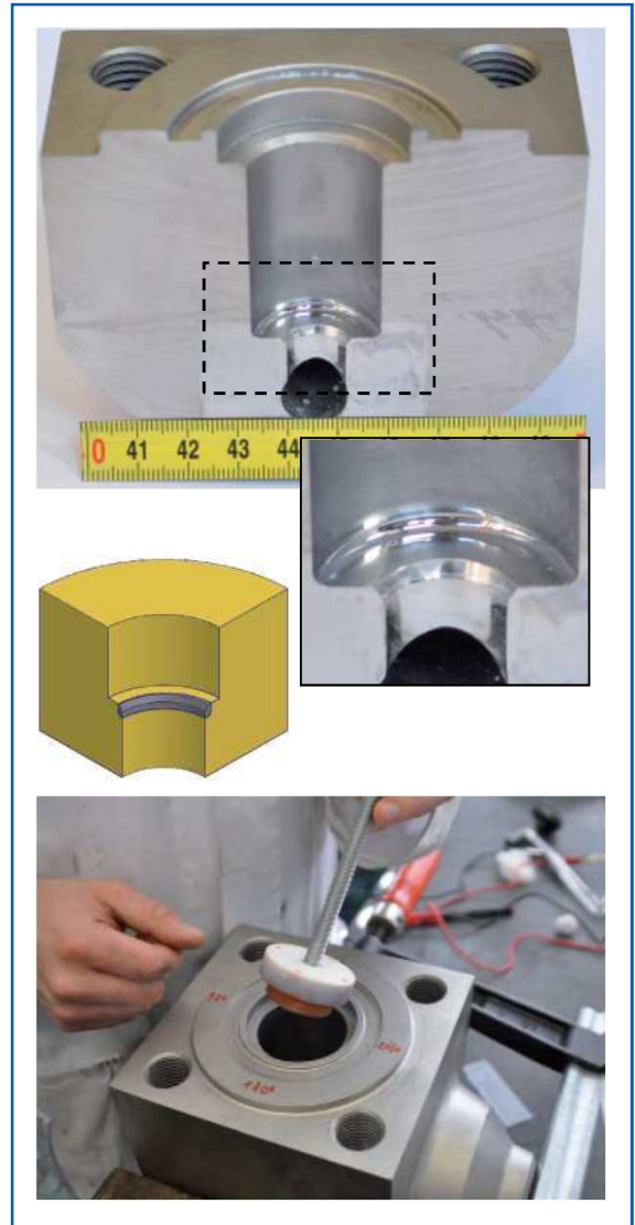
Investigation of small valves with special replica tools
