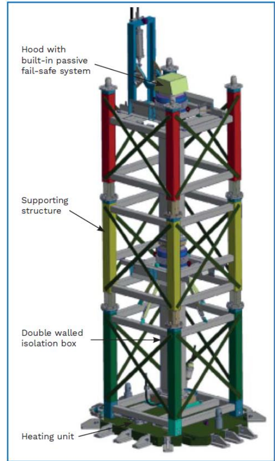
Mobile Box Sipping unit © Framatome
