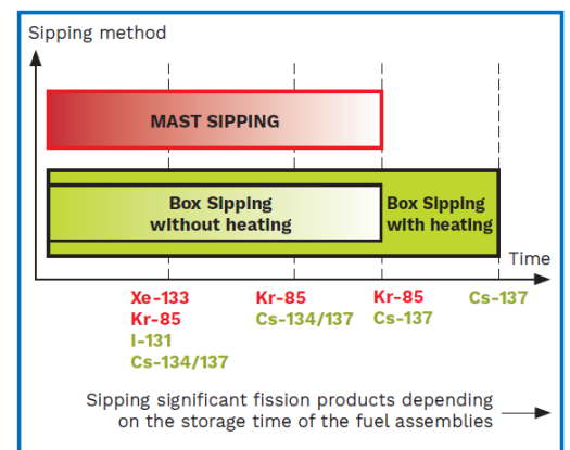
Sipping methods during outage and after long-term wet storage © Framatome
