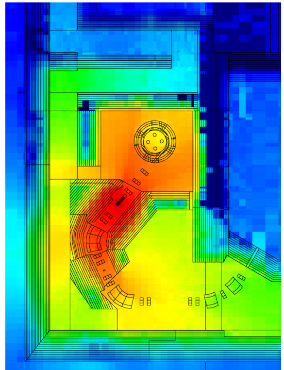
Fig. 1: Dose Distribution of Proton Therapy Center calculated with MCNP.
