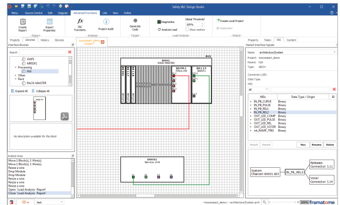
Function blocks diagram with TELEPERM XS Compact Design Studio. © Framatome
